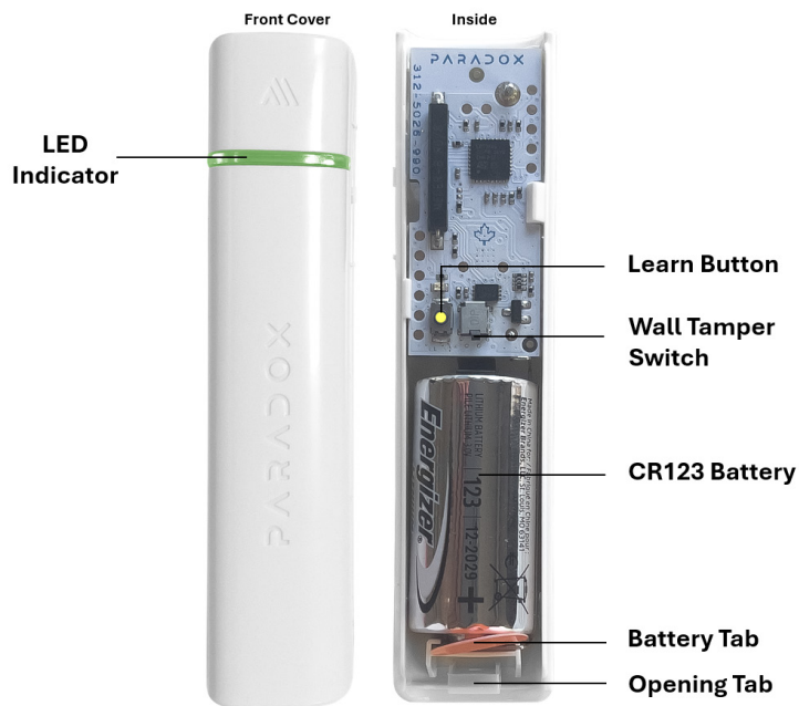
Components of DCT2M
